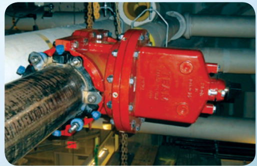
The InsertValve can be installed in any orientation on any type of pipe material.
